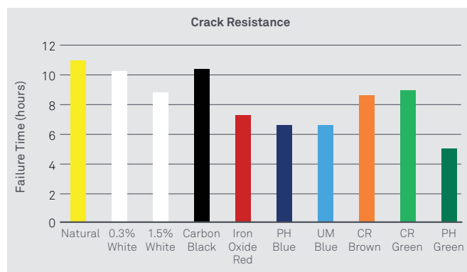
Figure 2. Crack resistance test results
