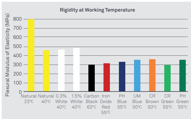
Figure 11. Rigidity at working temperatures
