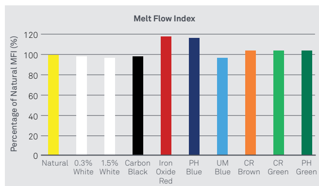
Figure 1. % MFI relative to natural PE
