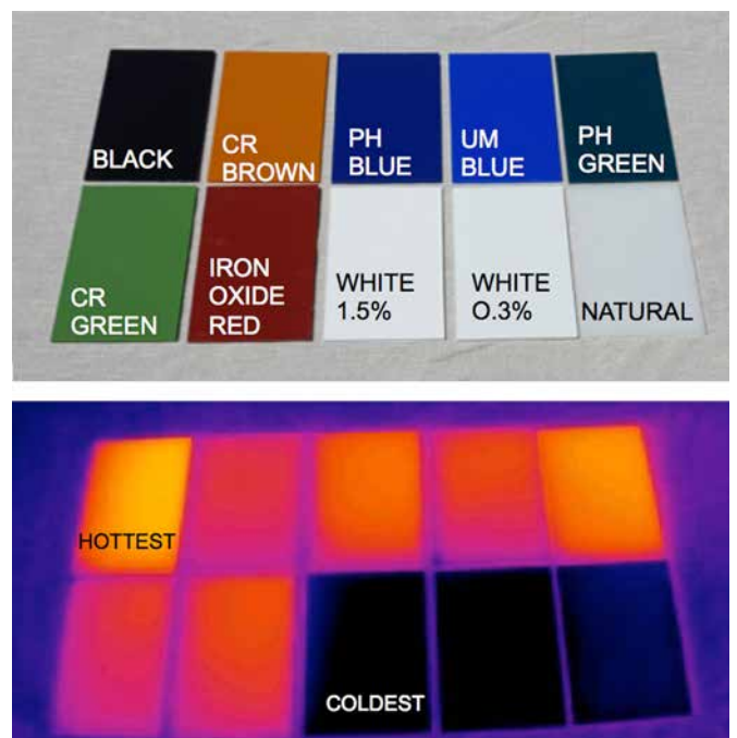
Figure 7. Thermal imaging of different pigments
