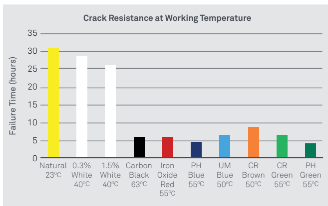
Figure 12. Crack resistance at working temperatures
