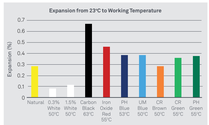
Figure 10. Expansion from 23°C to working temperatures
