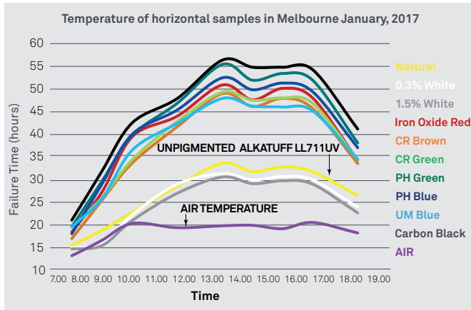
Figure 8. The different pigments generate different amounts of heat
