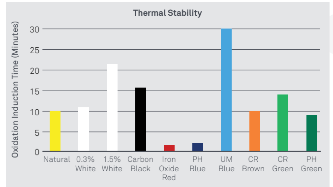
Figure 6. Thermal stability/surface oxidation test results
