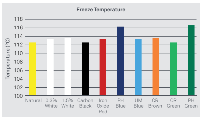
Figure 4. Freeze temperature test results
