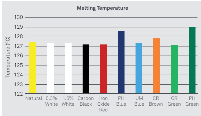
Figure 3. Melt temperature test results
